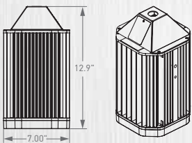
ALTUS With Pendant Mount (PDH). Weight: 19lbs
