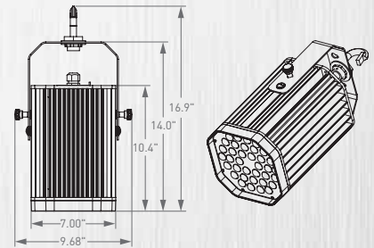
ALTUS With Free Hang Mount (FR). Weight: 19lbs
