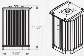
ALTUS With Ceiling Mount (CL). Weight: 19lbs
